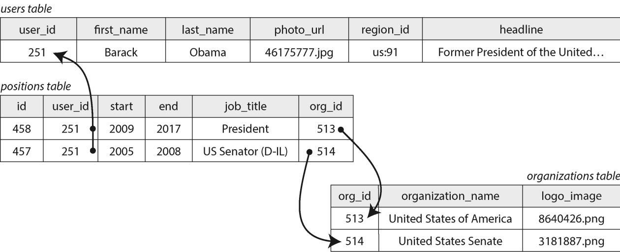
Figure 3-3. Many-to-many relationships in the relational model
